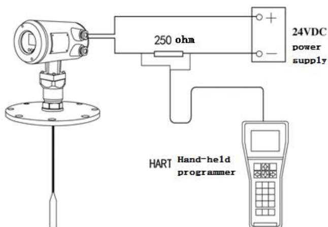
① HART handheld programmer ② Radar Level Transmitter ③ 250Ω resistor
