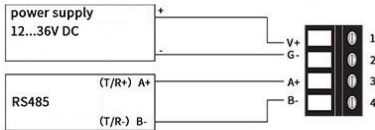
RS485 Output
